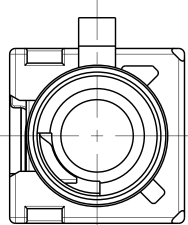
DETAIL F SCALE 5:1
