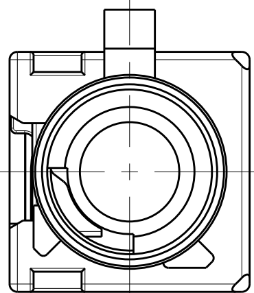
DETAIL M SCALE 5:1
