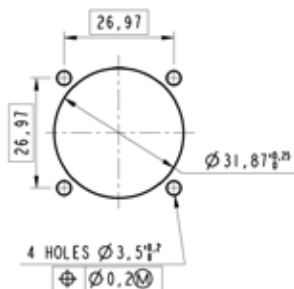
Panel Drilling
