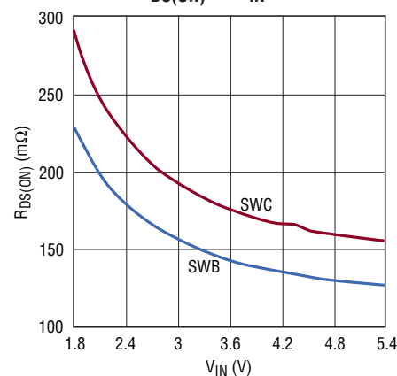
NMOS R_{\text{DS(ON)}} vs V_{\text{IN}}
