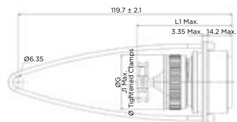
DBAS 978 With Straight Cable Clamp (059)
