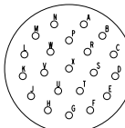
23-21 21 Size 16 Contacts
