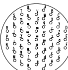
23-55 55 Size 20 Contacts
