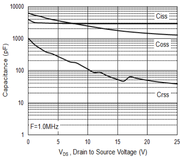
Fig.11 Capacitance
