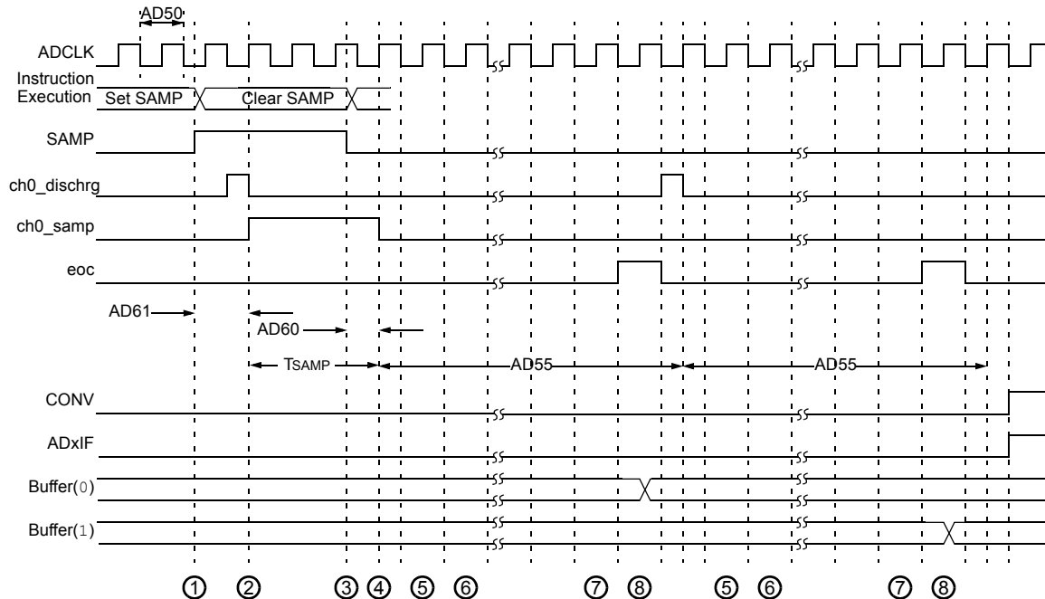
FIGURE 31-19: ANALOG-TO-DIGITAL CONVERSION (10-BIT MODE) TIMING CHARACTERISTICS (ASAM = 0, SSRC<2:0> = 000)
