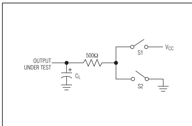
Figure 8. Driver Enable and Disable Timing Test Load
