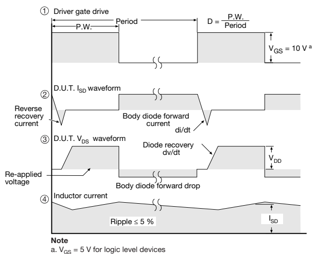
Fig. 14 - For N-Channel
