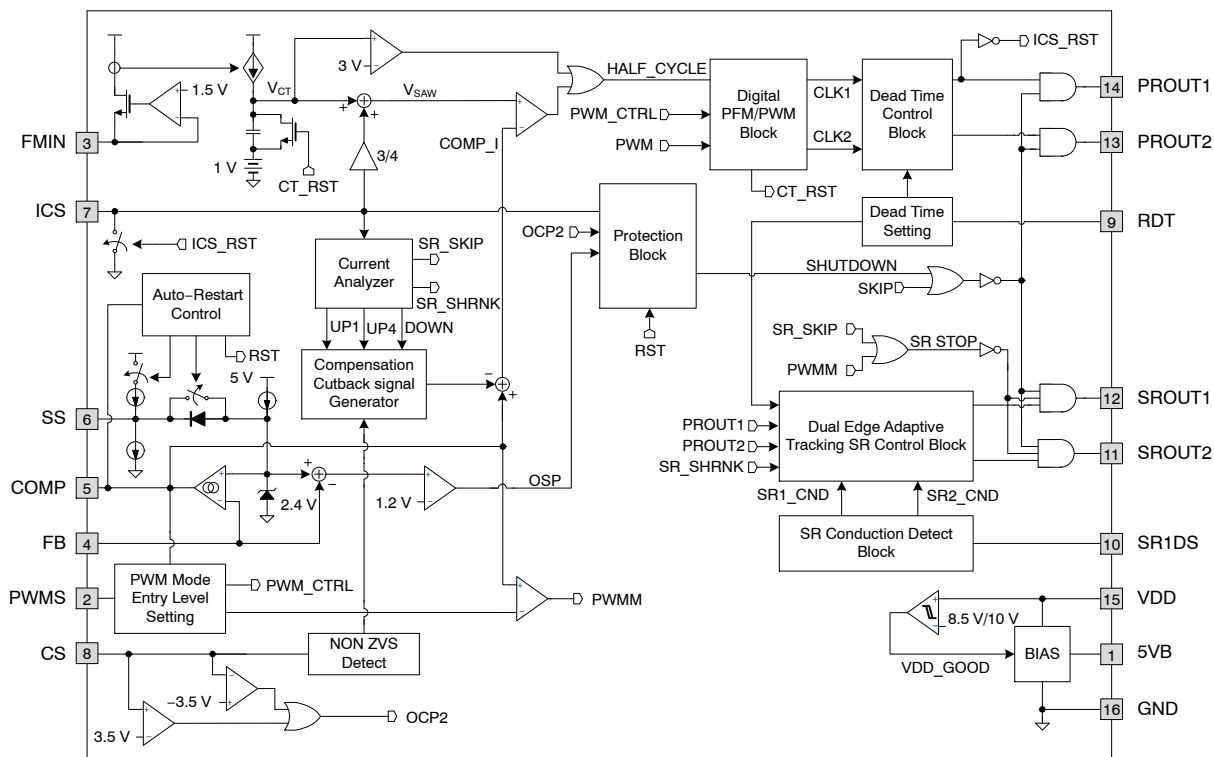
Figure 3. Block Diagram
