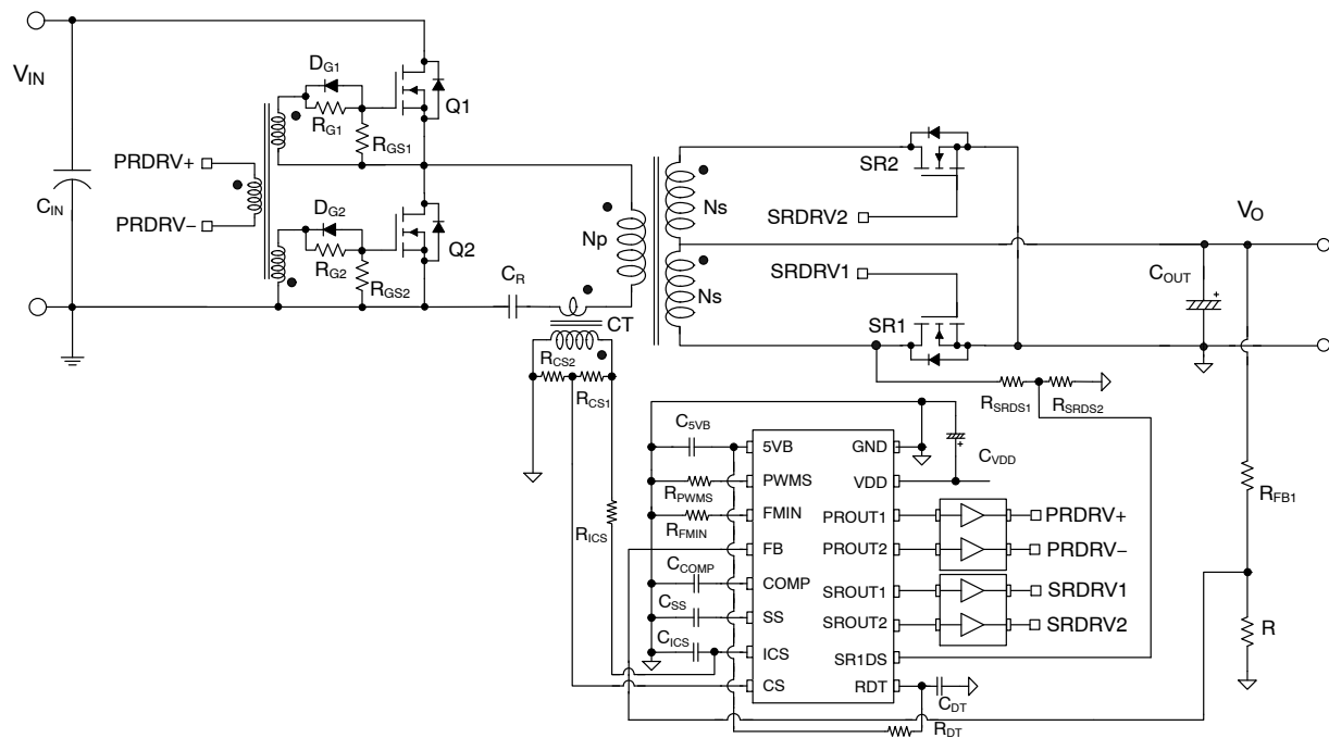
Figure 2. Typical Application
